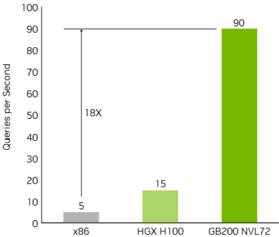
Database Join Query
